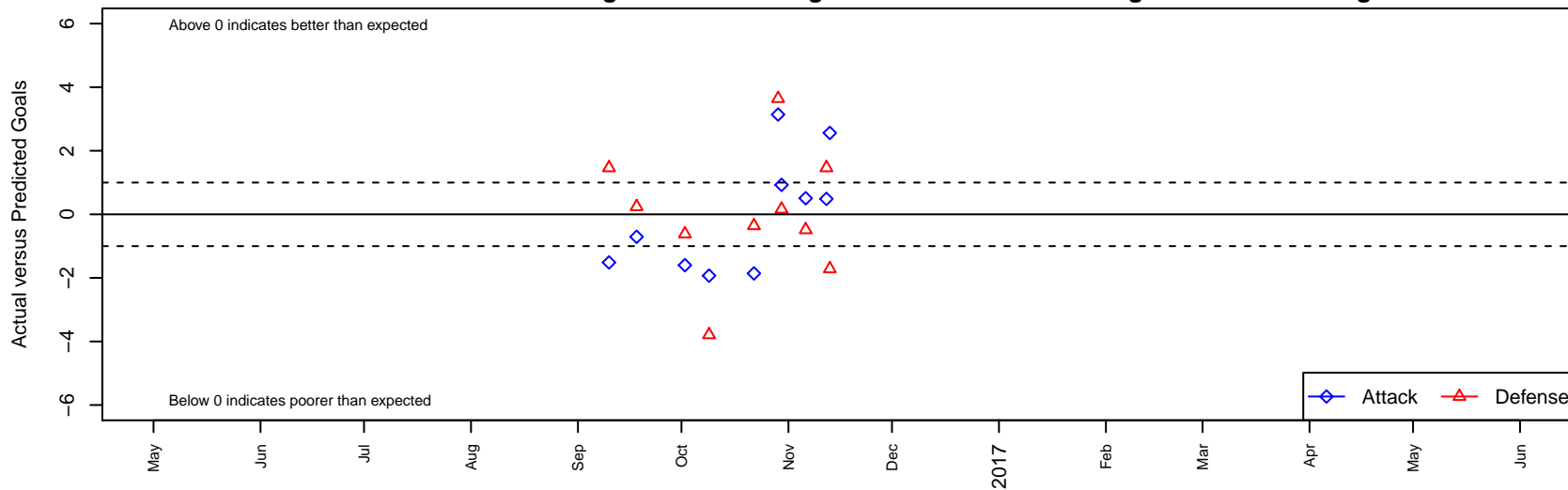
Liga Tlaxtli FC Guerreros B B02 Dots are actual minus expected GF (blue circles) and GA (red triangles). Blue line is smoothed change in attack strength. Red is smoothed change in defense strength.
